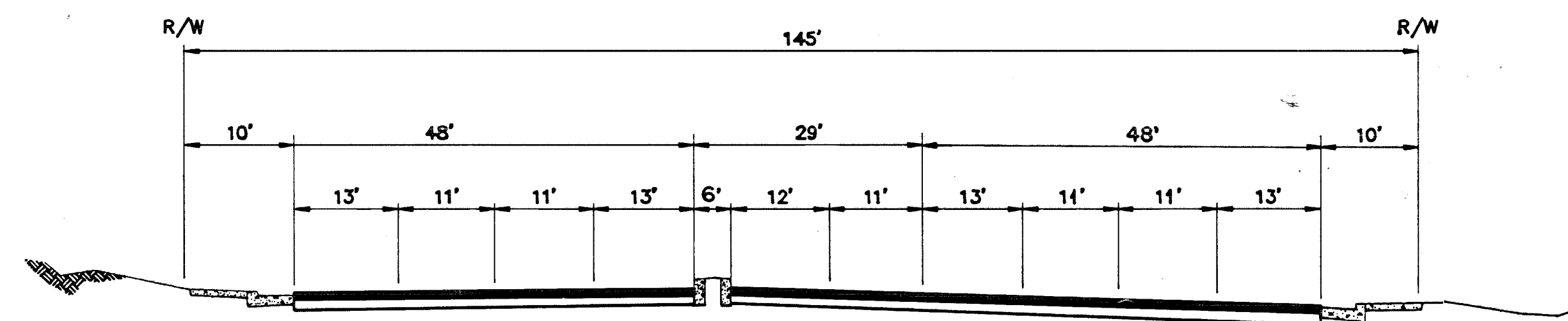
STANDARD SECTION (AT INTERSECTIONS) 145' R/W EIGHT MILE ROAD
