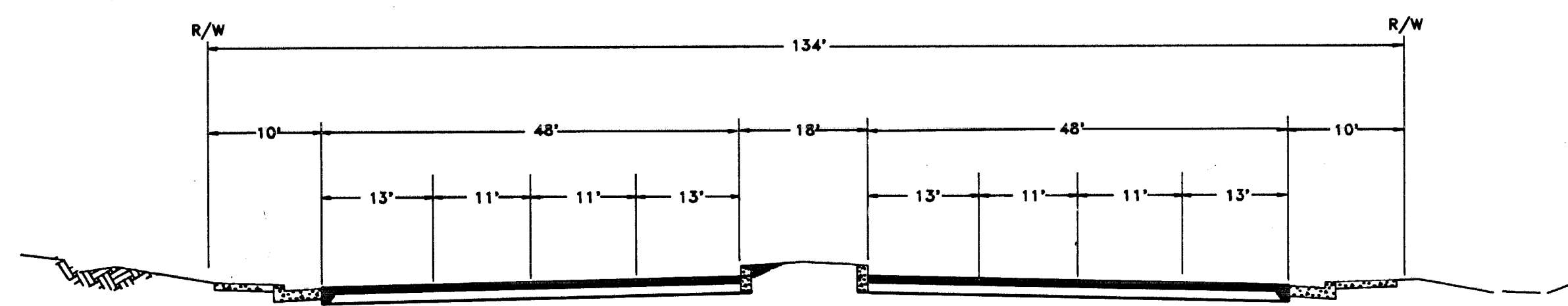
STANDARD SECTION 134' R/W EIGHT MILE ROAD
